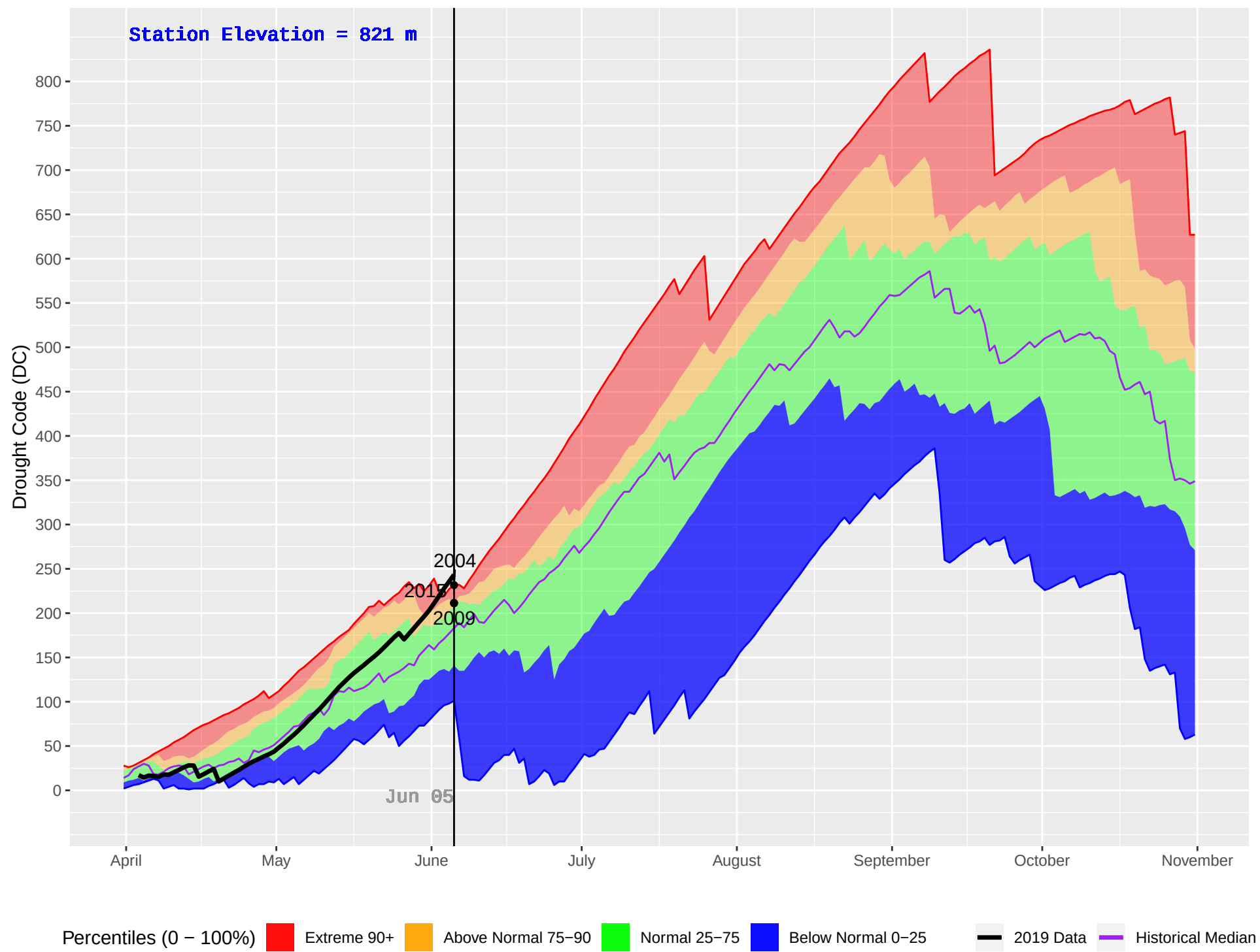
AKOKLI CREEK (838) : Historical (2003–2018) and Current (2019) Daily Drought Code (DC)
