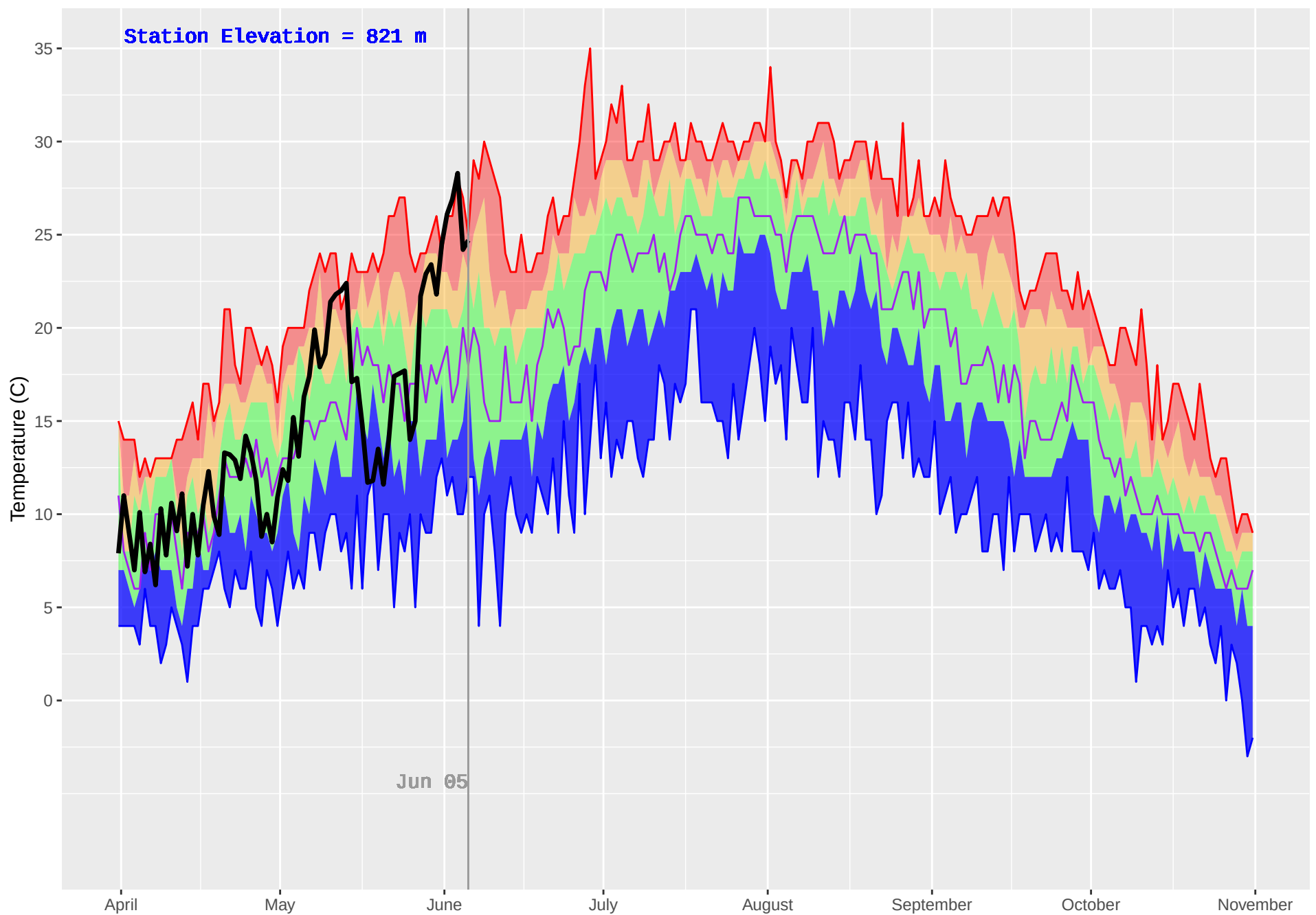
AKOKLI CREEK (838) : Historical (2003–2018) and Current (2019) Daily Temperature
