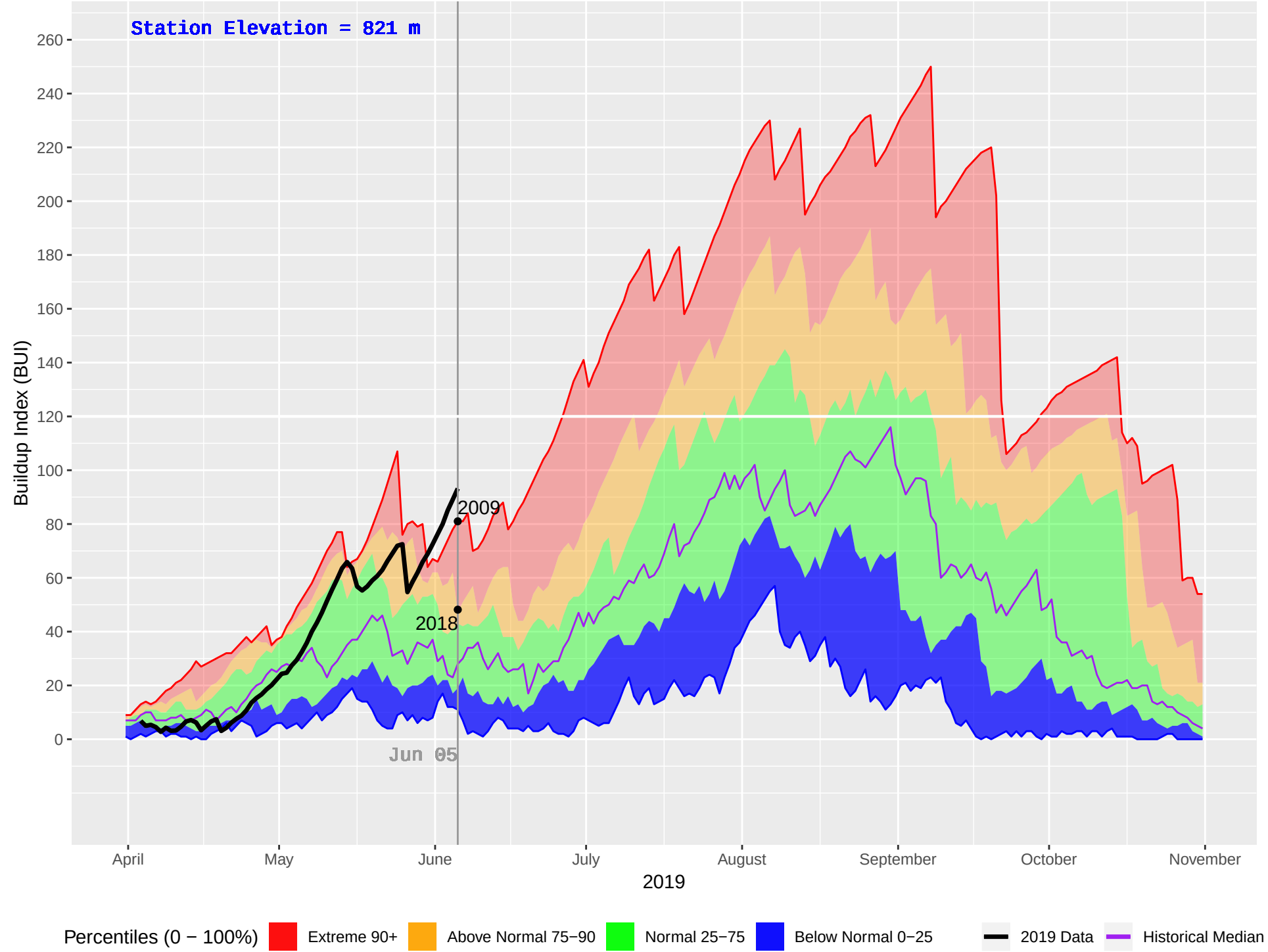
AKOKLI CREEK (838) : Historical (2003–2018), Current (2019) Daily Buildup Index (BUI)
