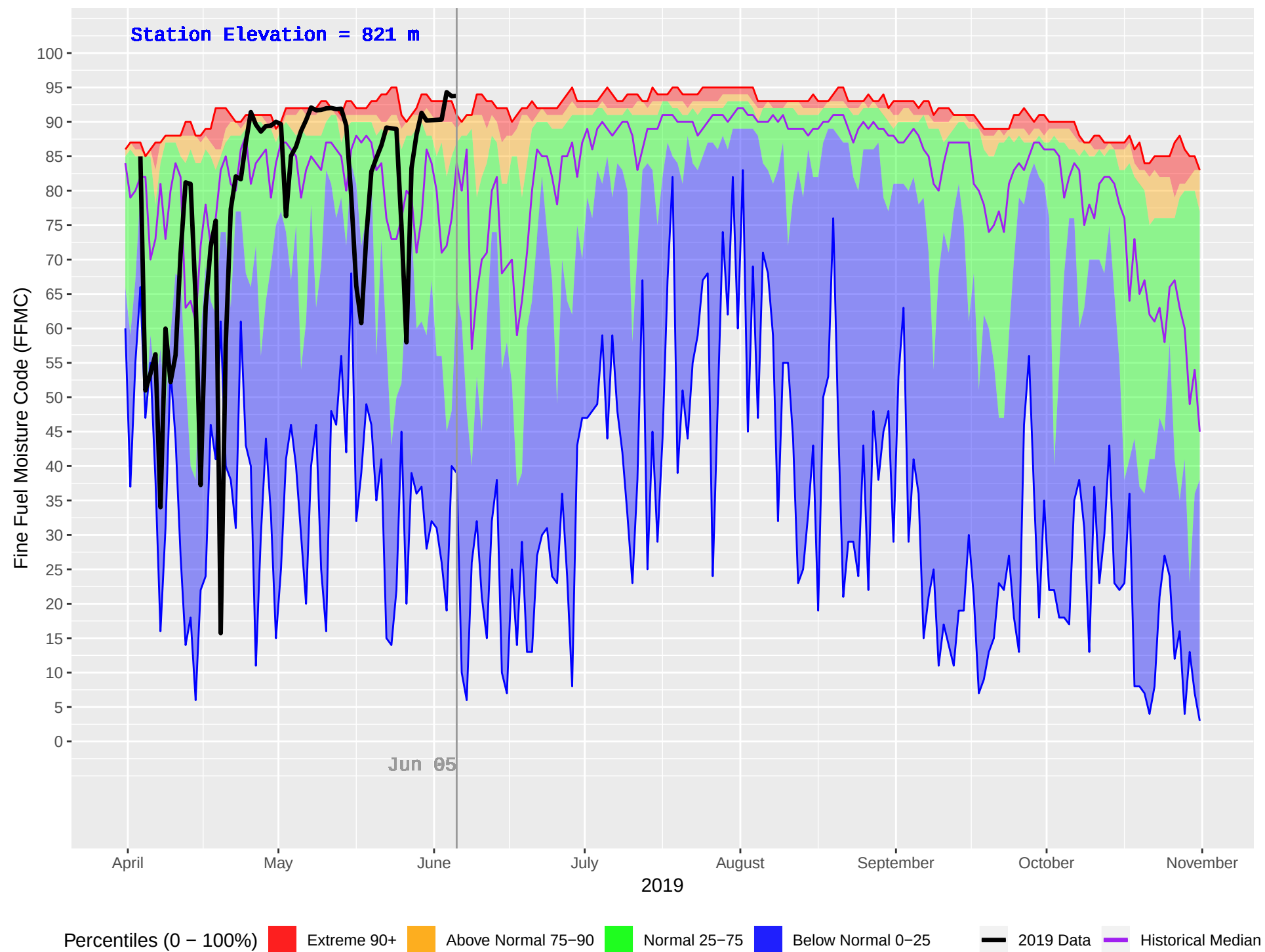
AKOKLI CREEK (838) : Historical (2003–2018) and Current (2019) Daily Fine Fuel Moisture Code (FFMC)
