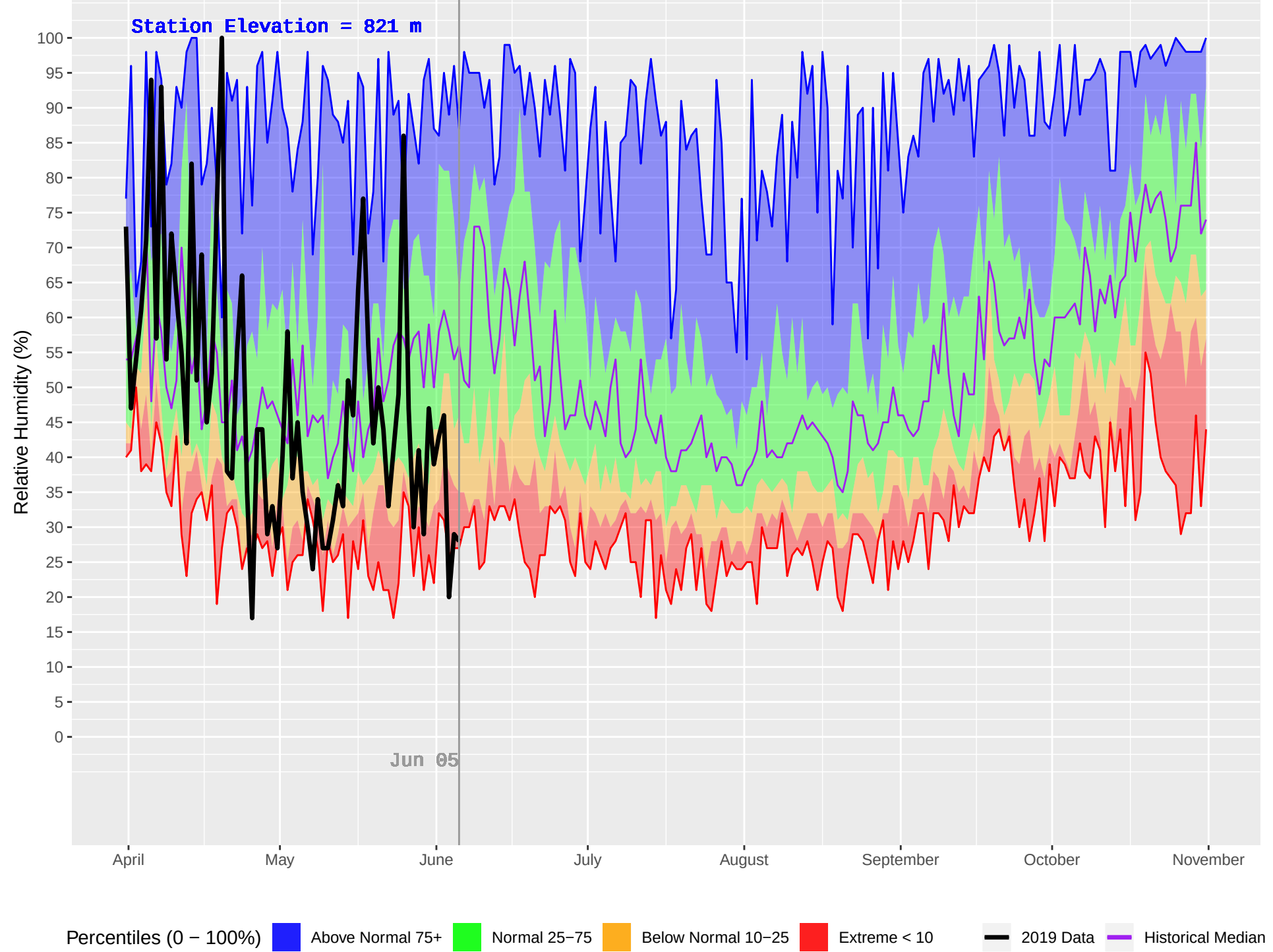
AKOKLI CREEK (838) : Historical (2003–2018) and Current (2019) Daily Relative Humidity
