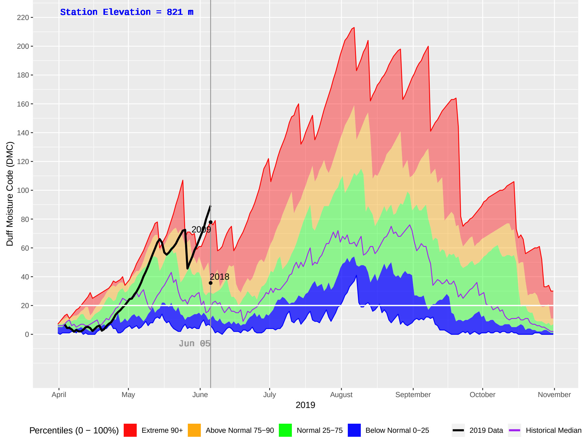
AKOKLI CREEK (838) : Historical (2003–2018), Current (2019) Daily Duff Moisture Code (DMC)
