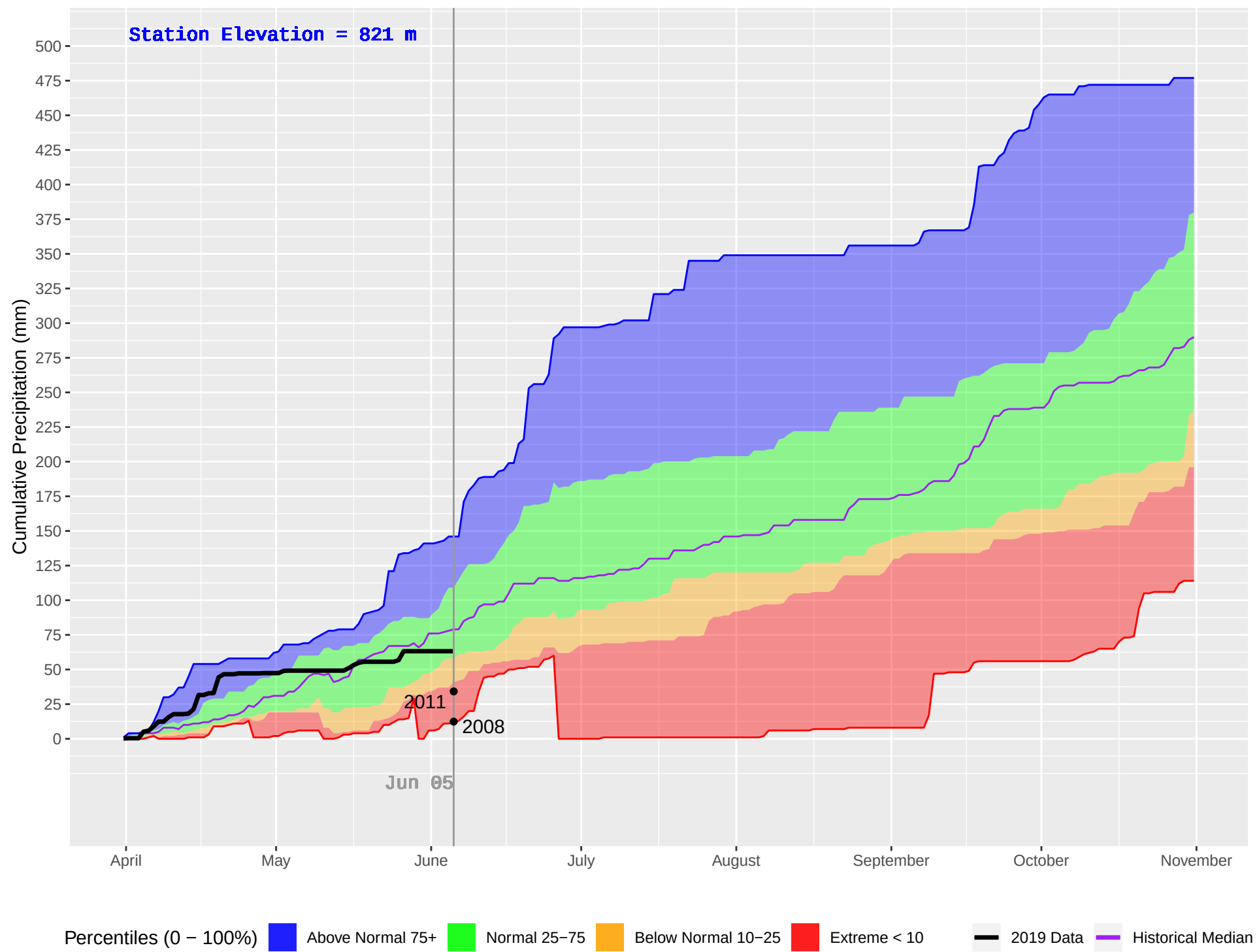
AKOKLI CREEK (838) : Historical (2003–2018), Current (2019) Daily Cumulative Precipitation
